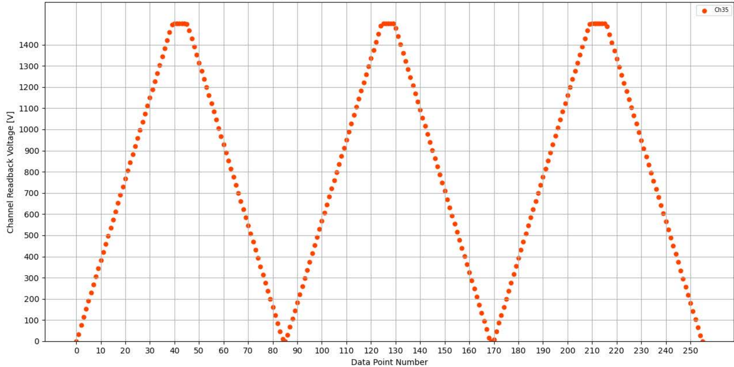
Voltage Ramp Test (Python) Bd #301, Slot #11, Ch #35
